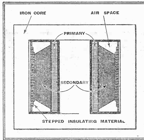
Fig. 9.—An HT secondary requires a modified form of winding technique. The air space is graded according to the working voltages of the layers.
