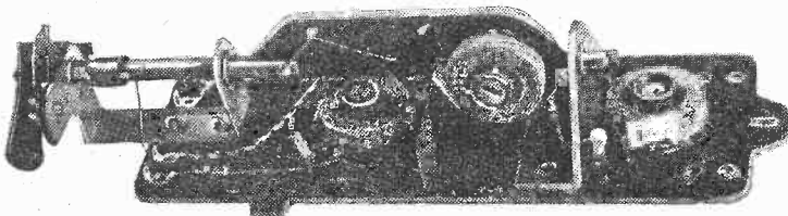
(Above) The new adjustable three-circuit IF band filter in the Körting "Amatus 40" and "Dominus 40."
