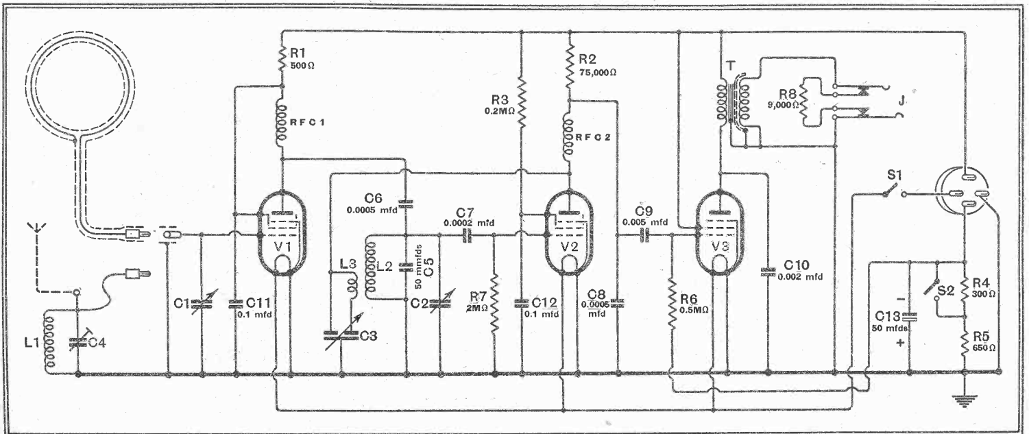
Circuit diagram showing values of components. The wiring should present no difficulty if this diagram is studied in conjunction with the photographs of the chassis.
