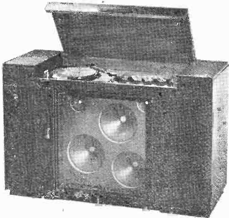
(Left) Siemens "Kammermusik-Gerät II," comprising a superhet receiver with 13 valves, 4 wave ranges (2 of which are short waves) and 5 loudspeakers.
