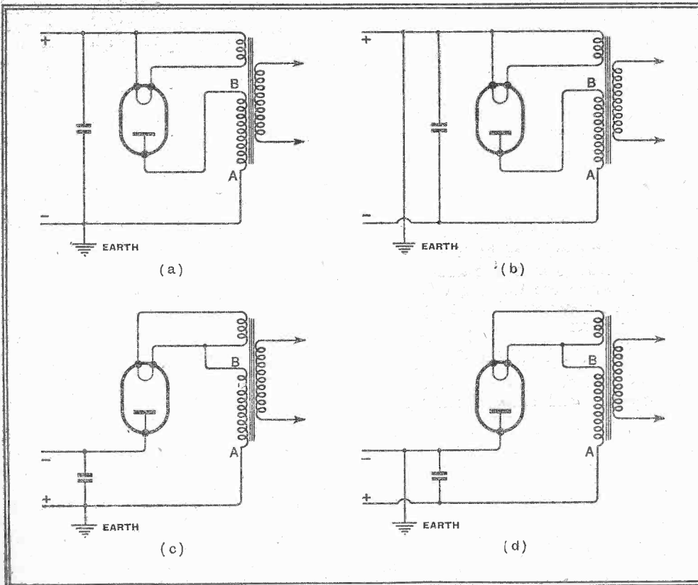
Fig. 5.—Several ways in which an HT rectifier can be arranged. The working voltages of the transformer windings are different in each case.
