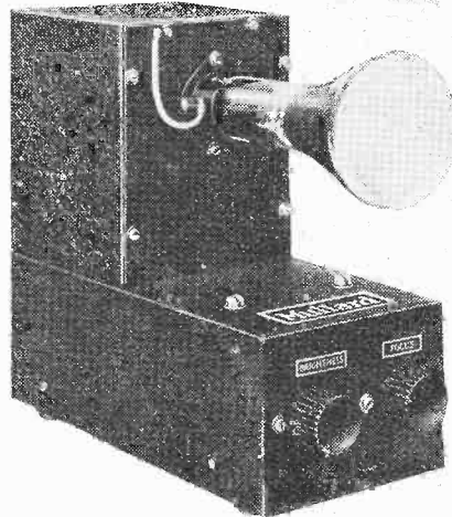
Mullard CR tube model Broo.
