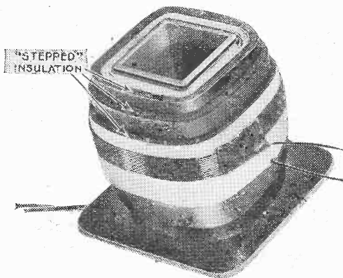
Fig. 8.—A photograph of an actual bobbin similar to the one shown diagrammatically in Fig. 7.
