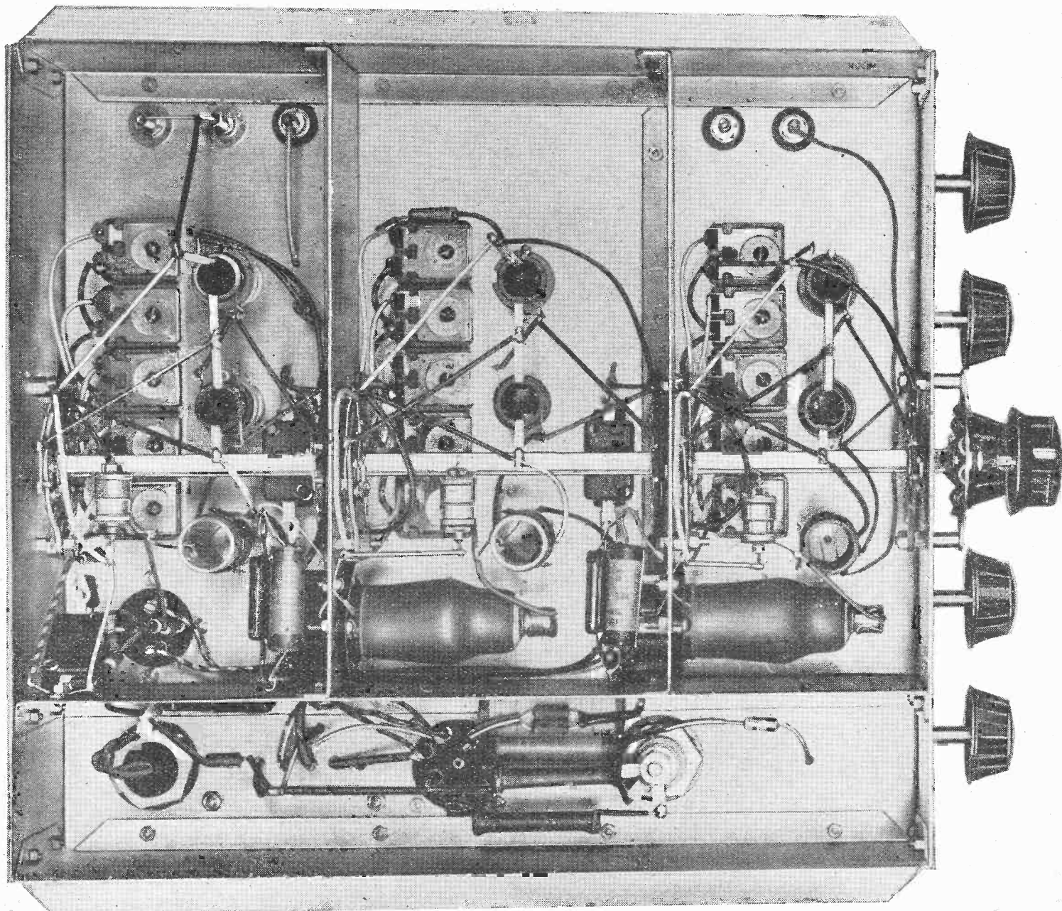
This underview of the receiver shows the RF valves mounted horizontally. This is done in order to secure very short leads on ultra-short waves.
