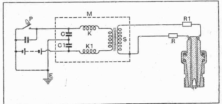
Interference suppression system for internal combustion engine.
