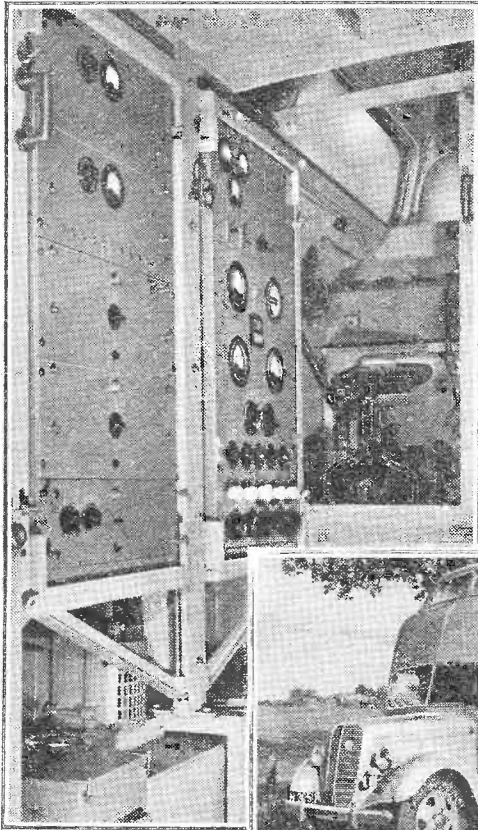
NORWAY'S RECORDING VAN incorporates a reporter's glass conning tower the interior of which can be seen above.
