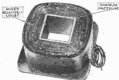
Fig. 2.—Considerable pressure is experienced by the wire at the corners of the bobbin. This tends to damage the insulating material.
