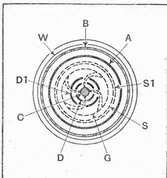
Sectional diagram of electrode arrangement in a magnetically controlled secondary-emission valve.
