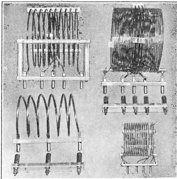
Plug-in type low-loss Denco coils.
