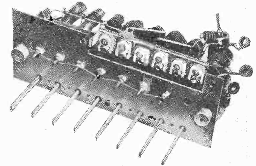
Wearite latest permeability push-button tuning unit.
