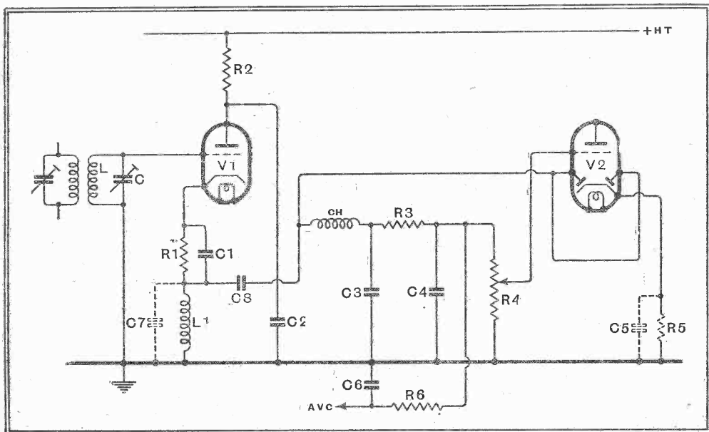
Fig. 7.—As an alternative to the arrangement of Fig. 6 the detector and AF stage can be combined by employing a diode-triode.
