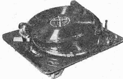
Garrard RC10 record changer.
