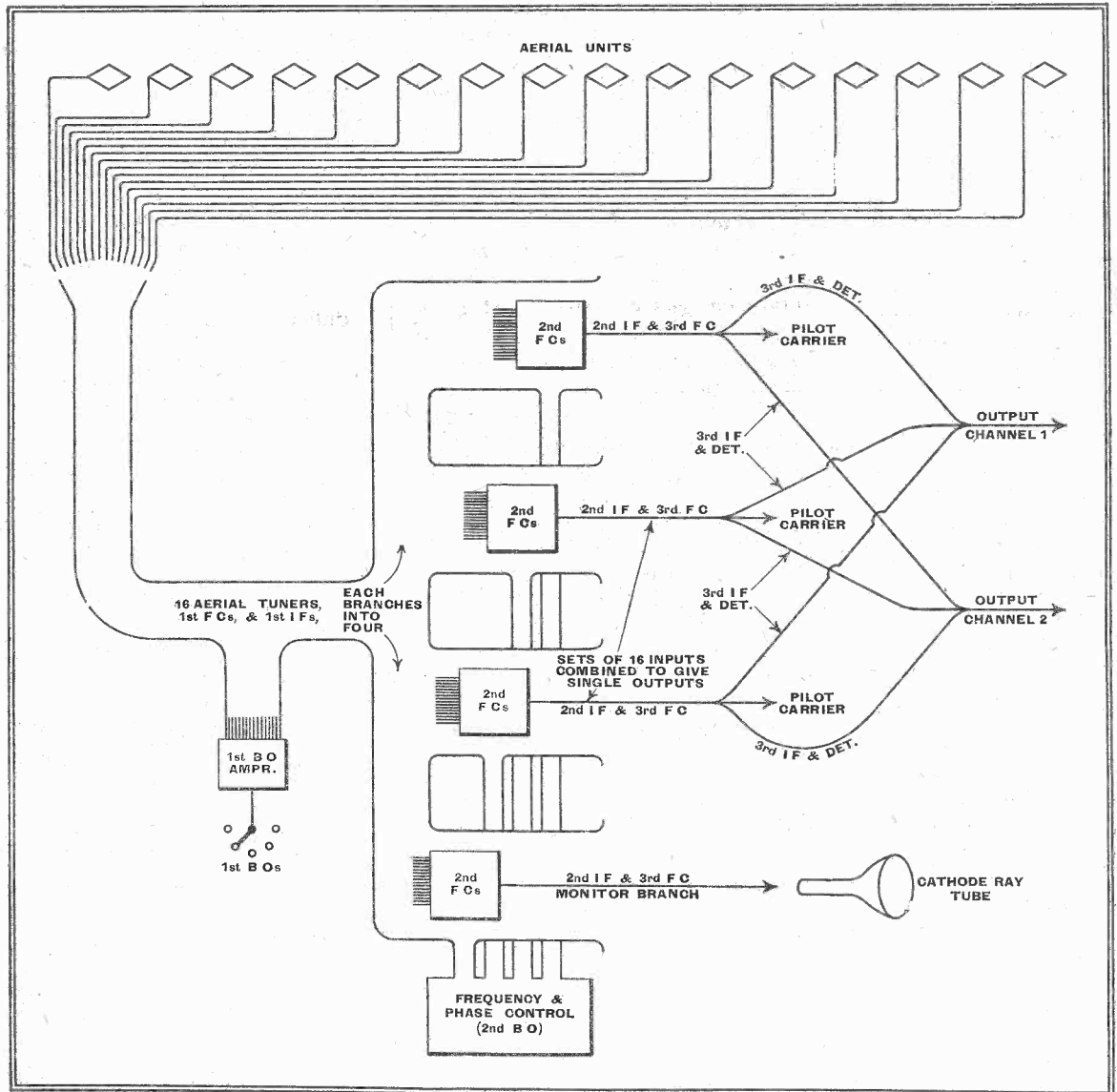
Fig. 2. How receiver paths, such as the one shown in Fig. 1, are bundled together, branching out and recombining, to obtain the special advantages of the Musa system.
