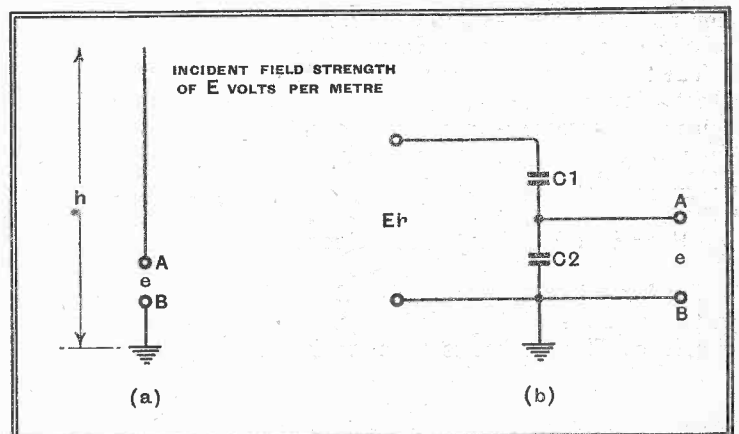
Fig. 2.—Diagram (a) represents a simple “Marconi” aerial, while at (b) is shown the equivalent circuit.
