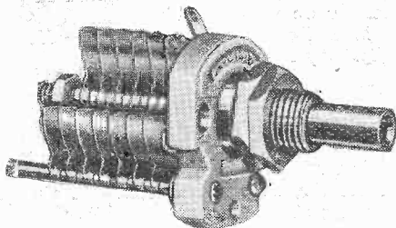
Miniature-type Polar condenser for ultra-short-wave circuits.
