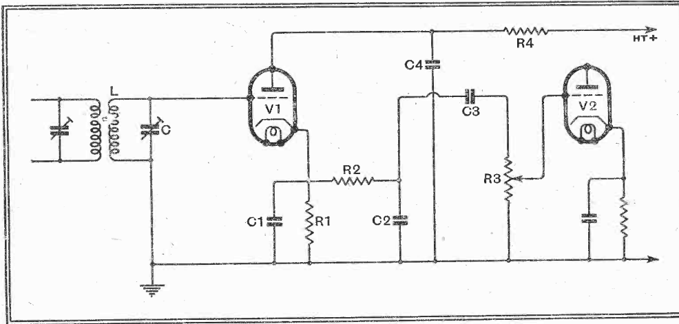
Fig. 4. The negative feed-back anode-bend detector has the load resistance in the cathode lead. Its efficiency is of the same order as that of the diode, but the input circuit is undamped; in fact, regeneration can be obtained.
