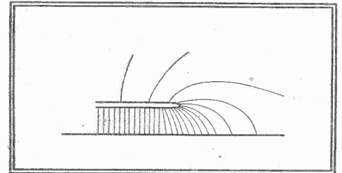
Fig. 7. Owing to the diverging field the electrical stress at sharp angles is much greater than the average.
