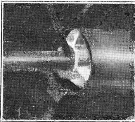
Close-up of one of the coaxial cables before anchoring flanges were put on, showing porcelain insulator and inner copper tube. This and the previous photograph were supplied by the Post Office Film Unit.
