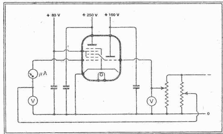
Fig. 3.—Typical measuring circuit used to obtain the static signal-grid-volts—grid-current curve of a triode-heptode.
