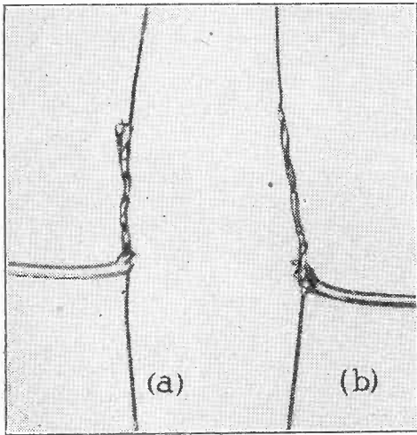
Fig. 4.—Illustrating how soldered joints can be a source of danger. Absence of roughness is very important.
