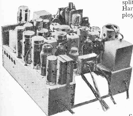
Chassis of Marconiphone television receiver.
