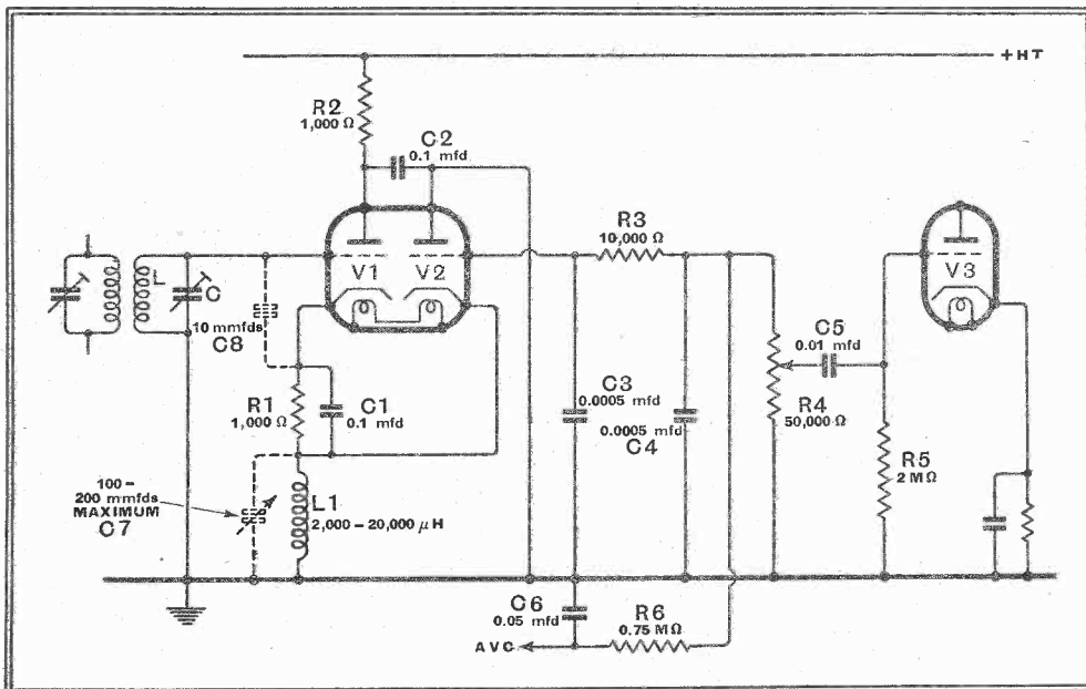
Fig. 8.—If separate valves are not used for each stage, the best arrangement is to employ a duo-triode as shown here. One triode section is used as a diode; the advantage over the diode-triode is that the cathodes are separate.
