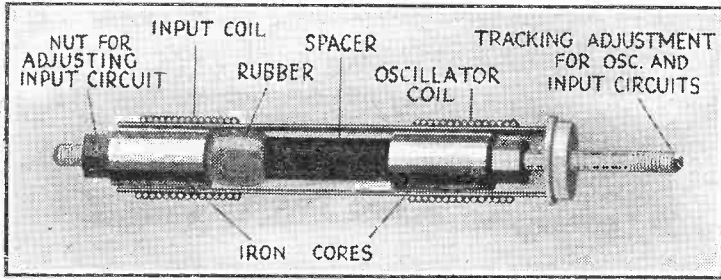
(Above) Iron-cored adjustable inductances for Telefunken push-button superhet.
