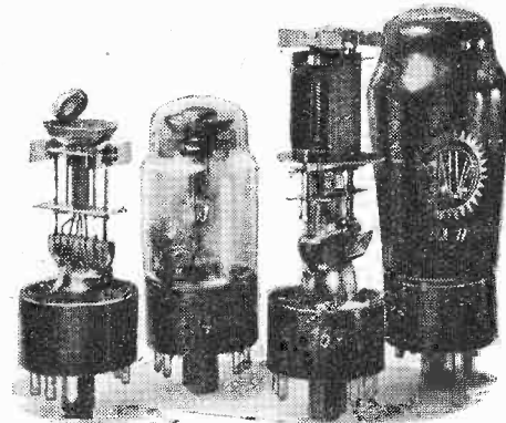
The new valves EM 11 and ECL 11. In the latter (right), from top to bottom can be seen the tetrode system, the triode system, the screening of the connections, and the constricted foot.
