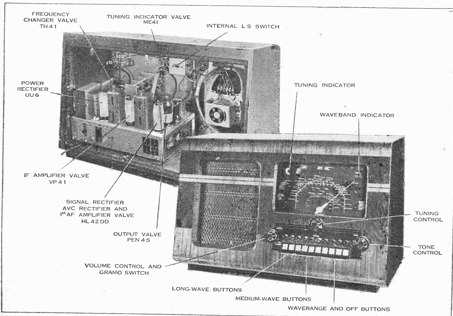
Layout of valves and controls in the R.G.D. Model 166. Trimmers for the station buttons are situated behind the moulded escutcheon. Aerial and oscillator circuits are adjusted simultaneously by a single set screw.
