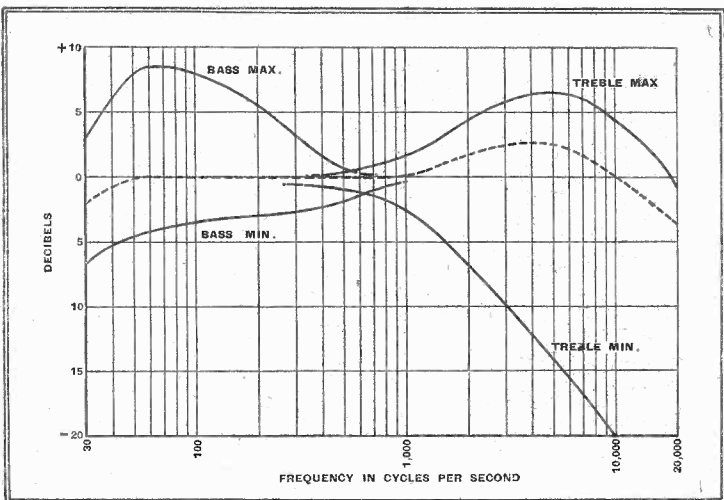
Frequency response of Grampian Type 385 amplifier. The dotted curve is for an arbitrary setting of the tone controls near their mid-positions.
