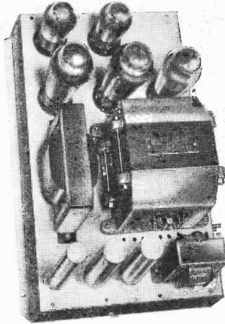
The layout of the power unit is clearly shown in this photograph.
