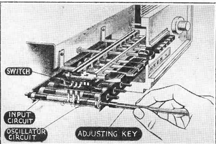
(Left) Details of permeability tuning system in Telefunken sets. By the action of the push-buttons a special oscillator circuit and preliminary circuit is switched in for each station.
