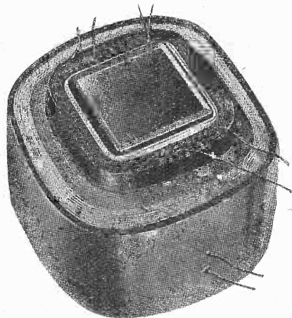
Fig. 10.—A photograph of the bobbin of the transformer specified for "The Wireless World" Magnetic Television Receiver. The outside insulation has been removed.
