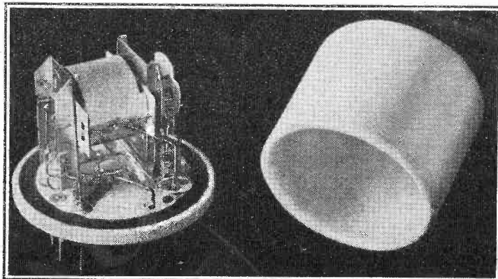
A CERAMIC ENVELOPE and base have been used in the construction by Hescho of this latest German valve of the same size and shape as the all-metal type. The high-frequency screening, in types where it is needed, is effected by spraying a thin layer of metal on to the inside of the Calit cover.
