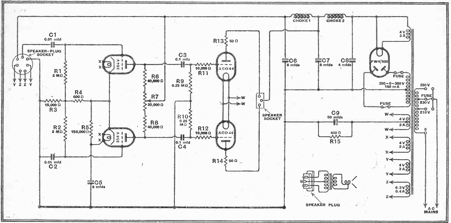
Fig. 2.—The AF amplifier is resistance-coupled push-pull, the necessary phase-reversal being obtained with the aid of the cathode resistance R3. The potentiometer R7 is provided for balancing.
