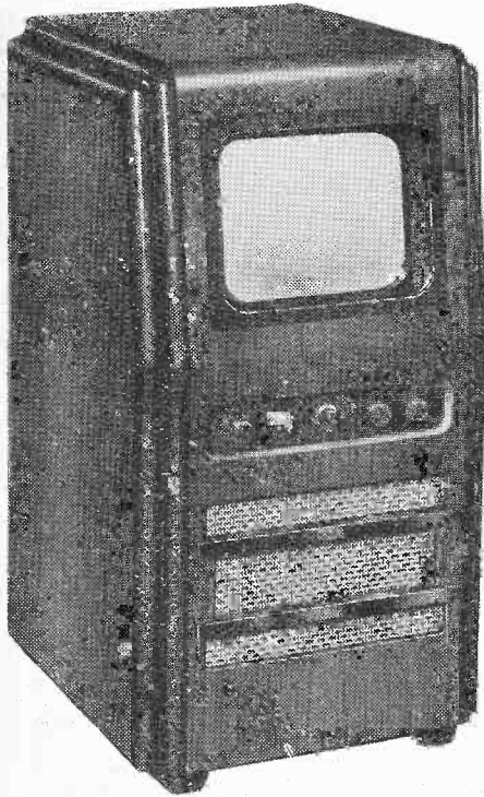
The Cossor 131 with 13½in. tube.
