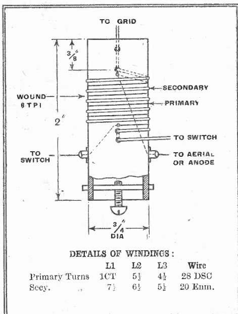
This drawing gives constructional details of the ultra-short-wave coils.
