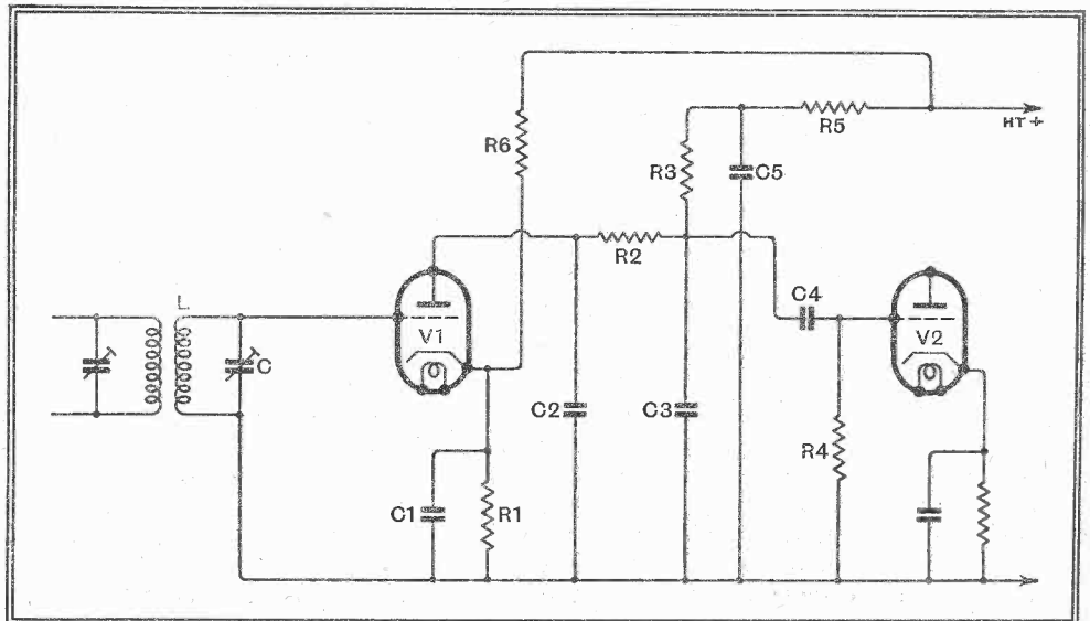
Fig. 3. With the anode-bend detector the input tuned circuit can be only slightly damped. The resistance R6 is often omitted.
