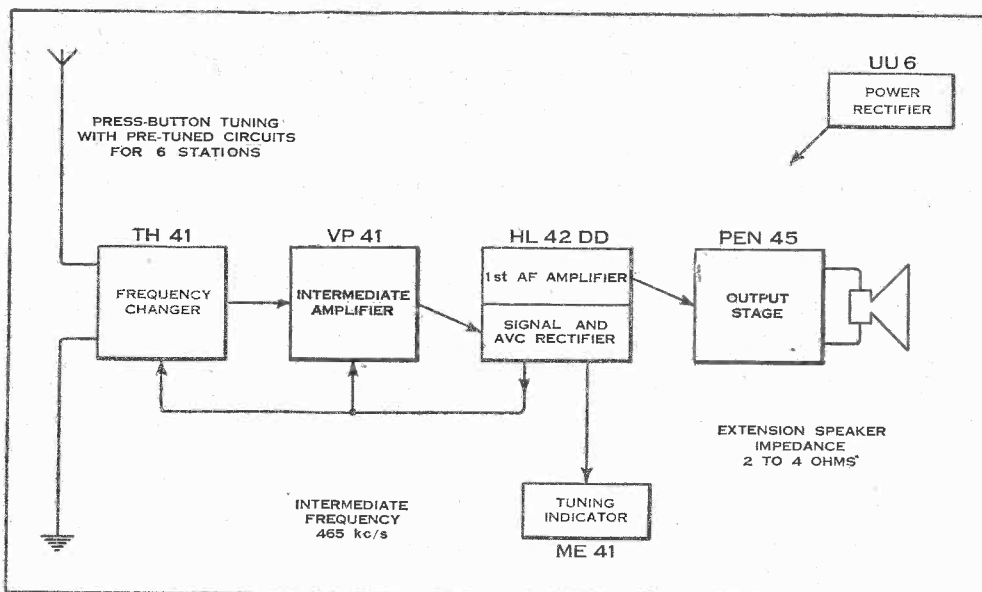
Schematic circuit diagram of the R.G.D. Model 166.
