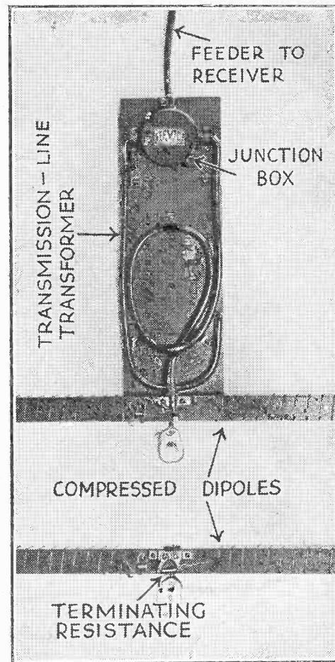
Part of the terminating dipoles; the top photograph shows the connection and transmission-line transformer between the aerial conductor and the feeder.
