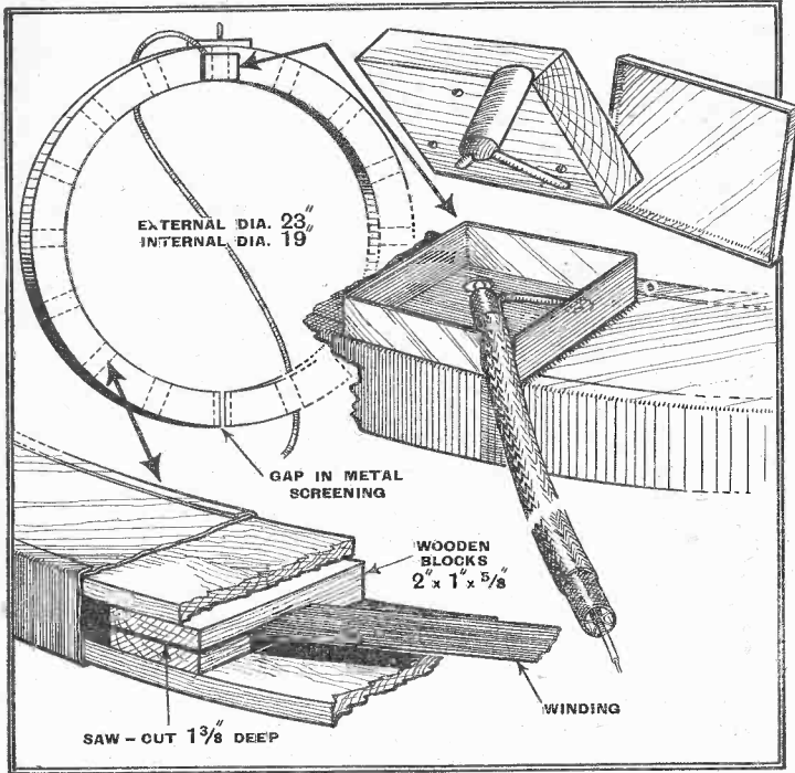
Leading dimensions and constructional details of the frame aerial. The winding consists of 26 turns of 22 SWG enamelled wire.
