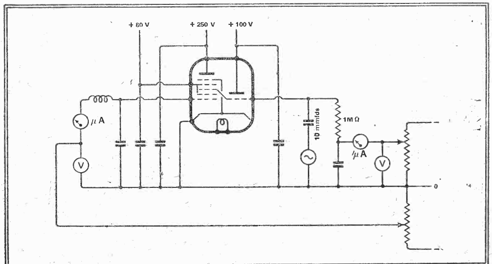
Fig. 5.—Measuring circuit to obtain I_{G1}=0 displacement curves as a result of very high frequencies impressed on G3 by a powerful signal generator.
