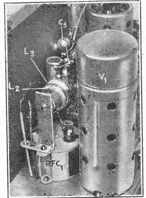
Details of RF coil mounting. The reaction coil connections are anchored to wires from the underside of the chassis and are easily reversed if the trial connections are made in the wrong sense.
