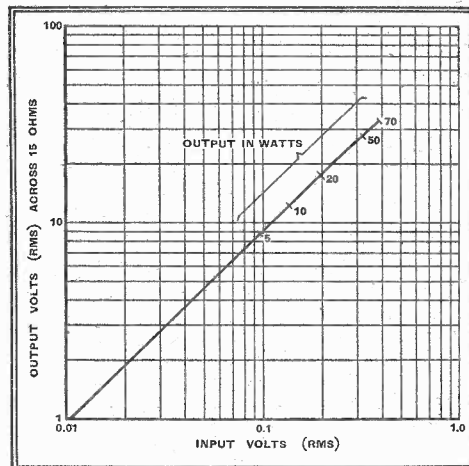
Input-output curve of the Grampian 50-watt amplifier taken on the pick-up input terminals. With direct connection to the grid of the first stage, full output is given for an input of 0.001 volt.
