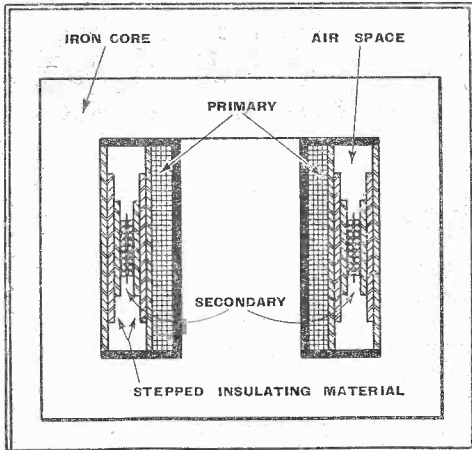
Fig. 7.—Showing how an LT secondary, working at high-potential, can be satisfactorily insulated. The points to note are mentioned in the text.
