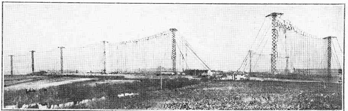
The Beam wireless stations now constitute an important link in the chain of Empire communications. This photograph shows the multiple aerial system at the Dorchester station, operated by Cable and Wireless, which recently established a record by transmitting 1½ million words in a week.
