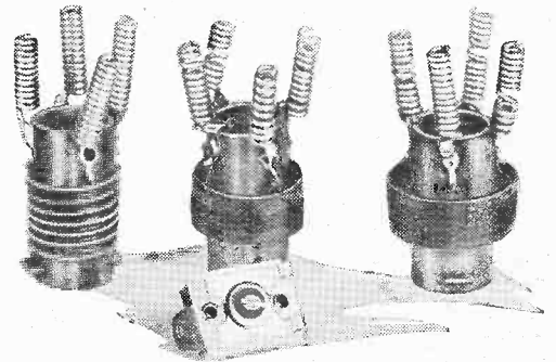
New unit coils with trimmer made by Bulgin.
