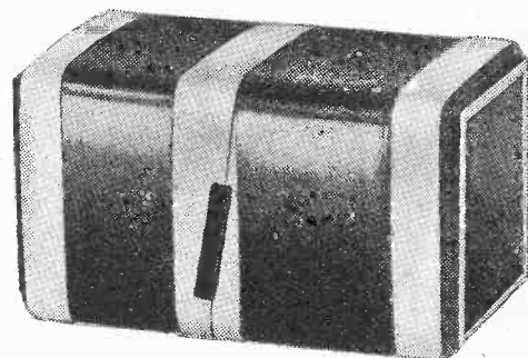
Fig. 3.—Joints must not upset the smoothness of the layer. A lump will result in local pressure and risk of breakdown.
