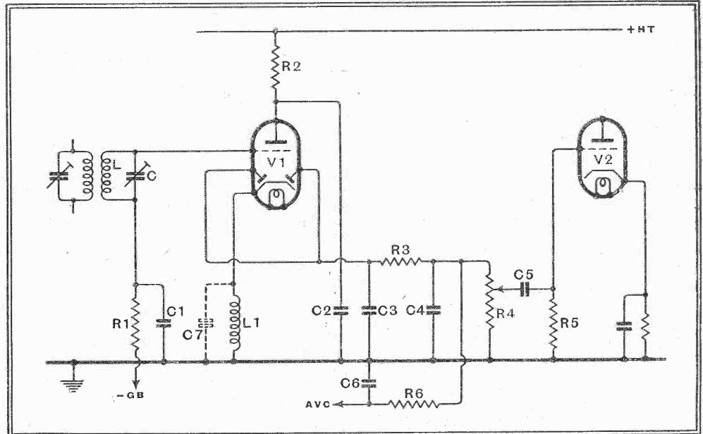
Fig. 6.—The detector and cathode follower can be combined by using a diode-triode as shown here.
