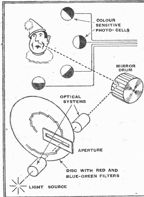
Fig. 4.—This drawing illustrates the transmitting system used in the recent demonstration. Spotlight scanning is employed.
