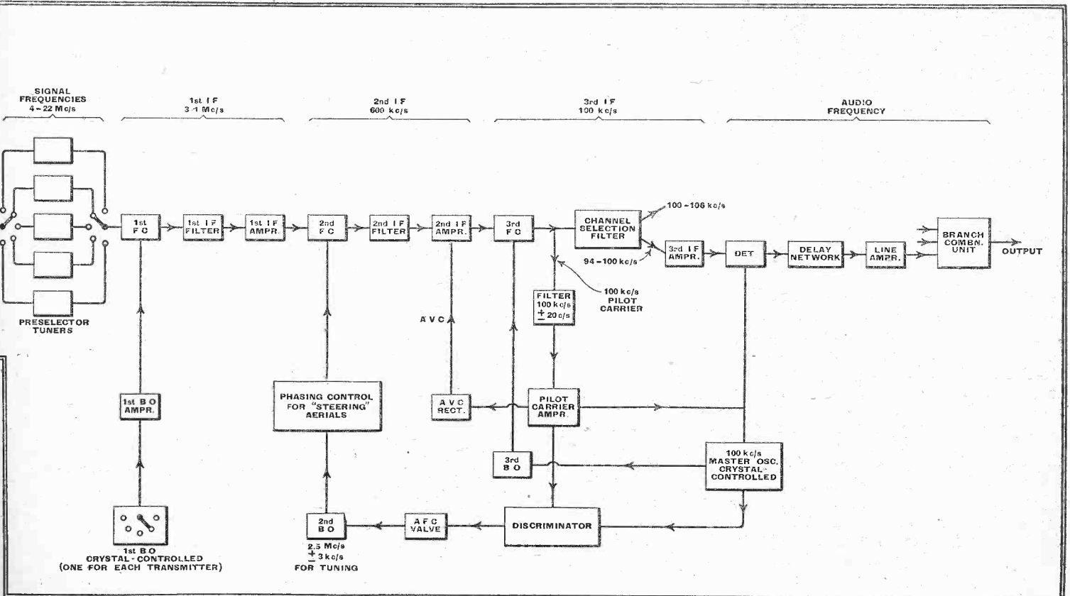
Fig. 1.—One complete receiver path from aerial to output. The direct signal path runs across the top of the diagram: the parts hanging from it are heterodyne (beat) oscillators and other frequency controlling accessories. Some of these are very complicated. Abbreviations: FC, frequency changer; BO, beat oscillator; IF, intermediate frequency; AFC, automatic frequency correction; AVC, automatic volume control.
