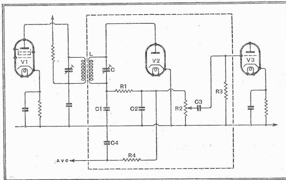
Fig. 1. This diagram shows the usual arrangement of a diode detector V_2 between an IF stage V_1 and an AF amplifier V_3 .
