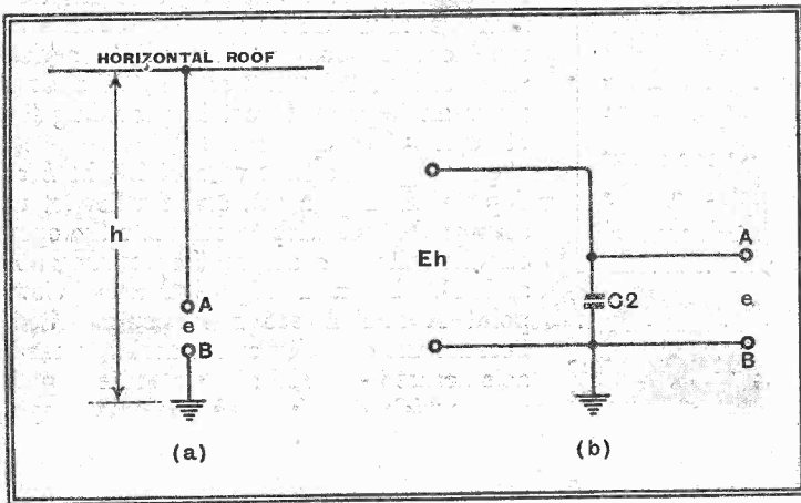
Fig. 3.—A “Marconi” aerial with a horizontal roof. Subject to restrictions mentioned in the text, diagram (b) represents the equivalent circuit when the roof is infinitely large.
