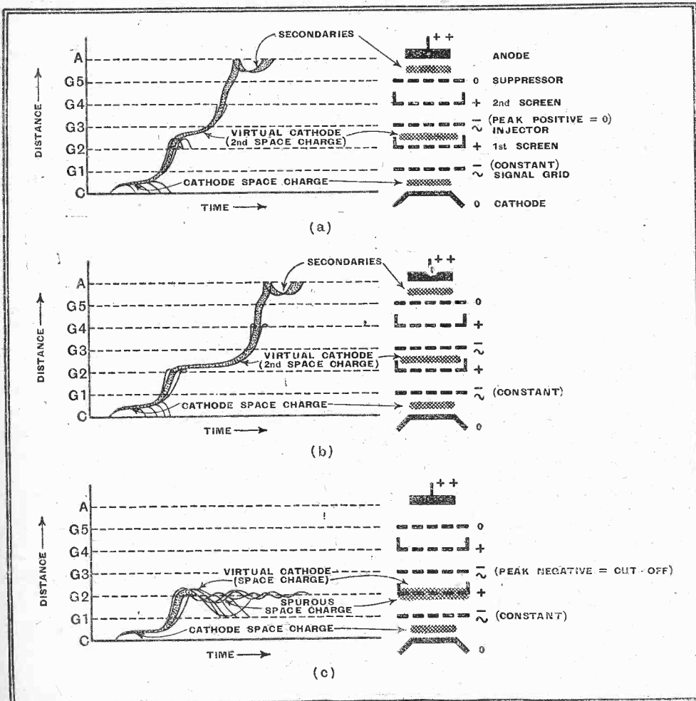
Fig. 1.—These rather unusual time-distance diagrams show the behaviour of the electron stream inside the heptode mixer path of a triode-heptode valve. (a), (b) and (c), correspond to the cardinal operating points of the heterodyne injector-grid voltage wave, shown in the lower half of Fig. 2.
