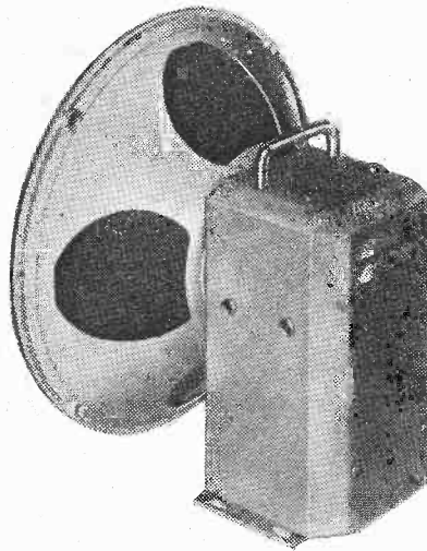
Goodmans P12 energised loud speaker.
