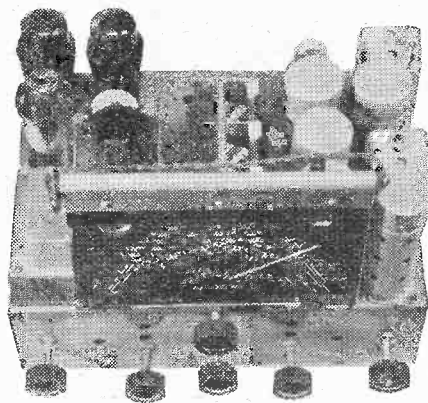
Armstrong Model SS10 "superhet-straight" receiver.
