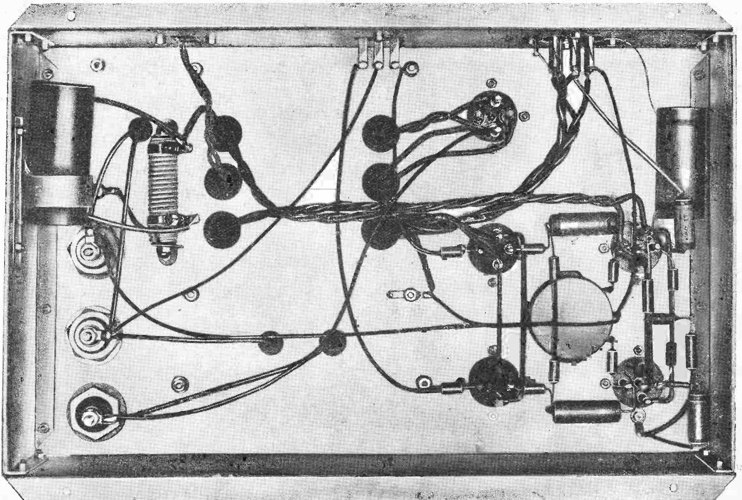
This photograph gives full details of the construction and wiring of the power unit.
