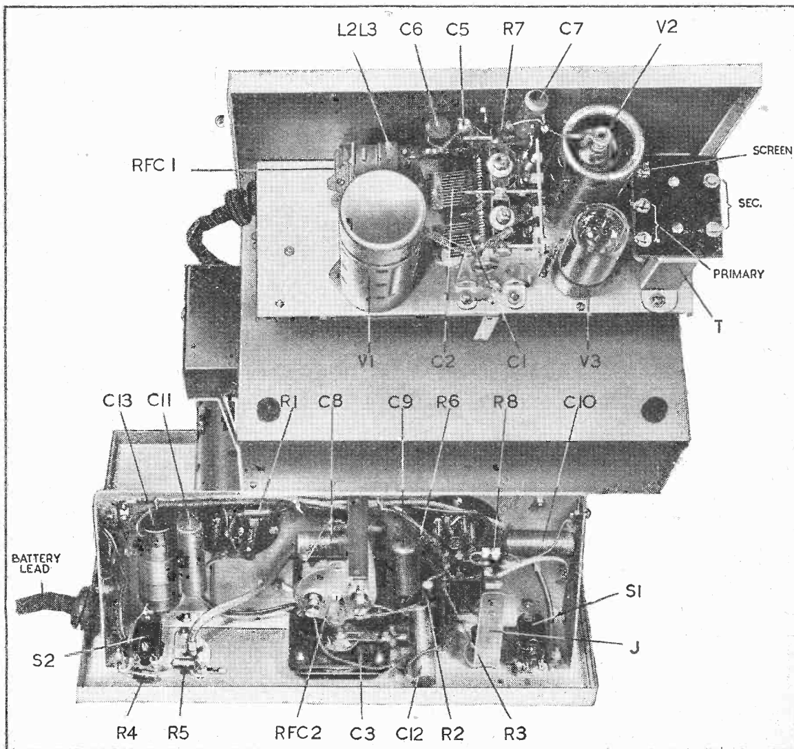
Views showing layout of components above and below the chassis shelf. Each part is lettered to correspond with the circuit diagram, and the wiring is quite straightforward.
