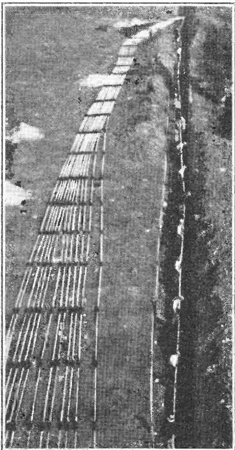
Burying coaxial cables used to connect the sixteen trapezoidal aeri-als of the Post Office MUSA system at Cooling to the receiver described in this article.
