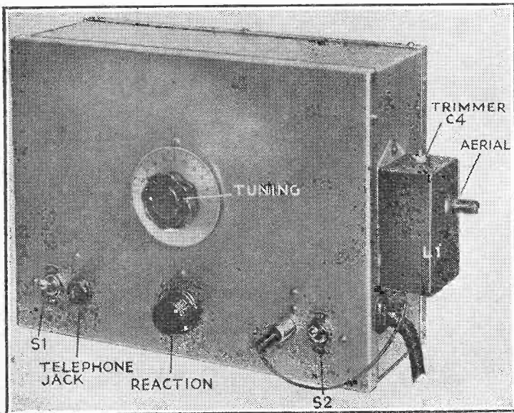
Layout of controls on the front panel. The auxiliary aerial circuit is shown connected to the frame aerial socket ready for use with a short external aerial.
