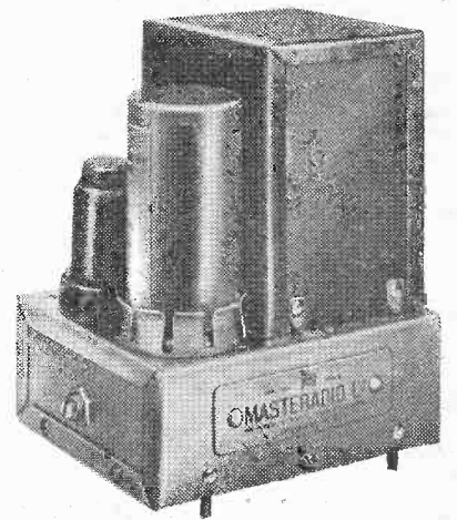
Vibrapack unit with adjustable voltage control made by Masteradio.
