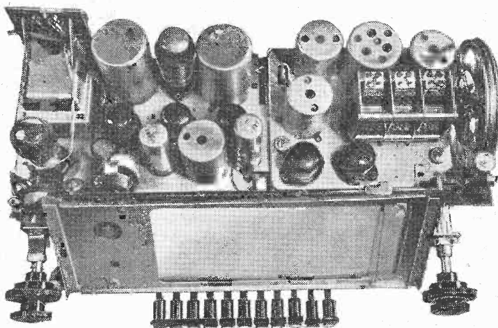
(Above) The new adjustable three-circuit IF band filter in the Körting "Amatus 40" and "Dominus 40."
