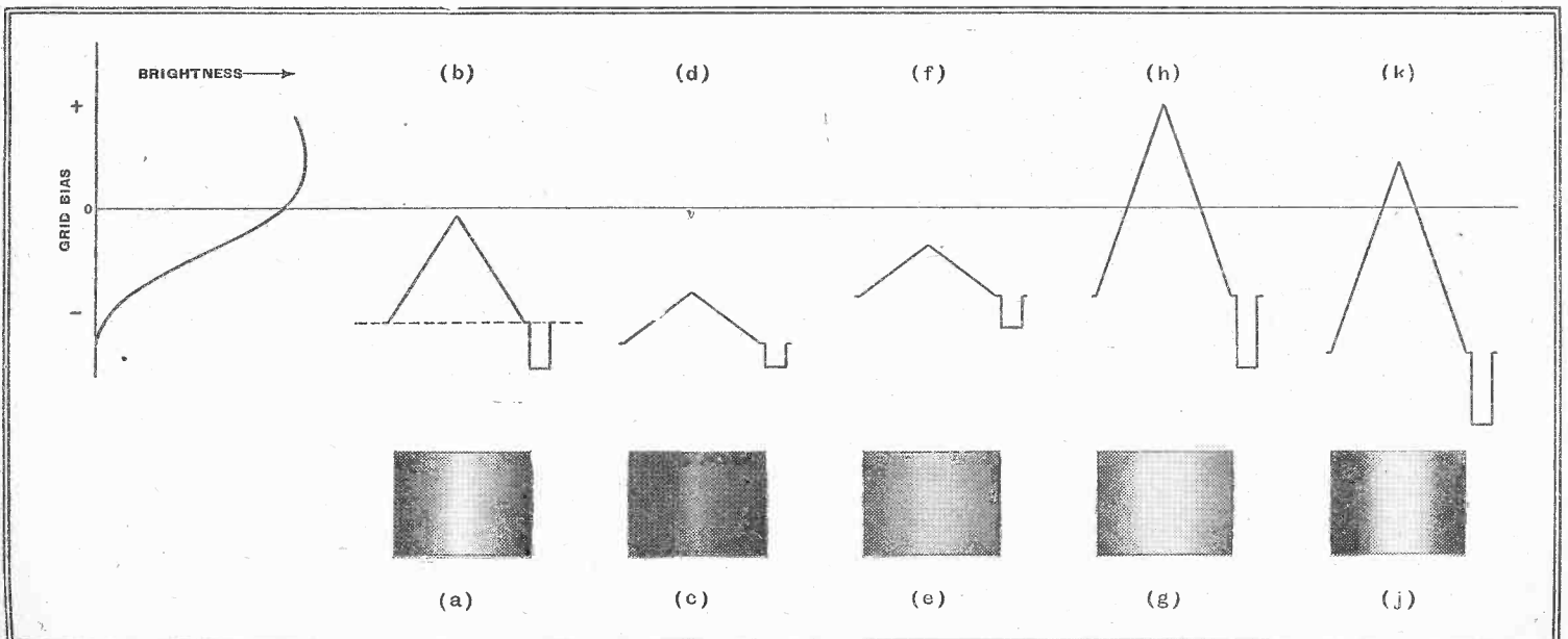
Illustrating the effect of operating the Brightness and Contrast controls of a television receiver.
