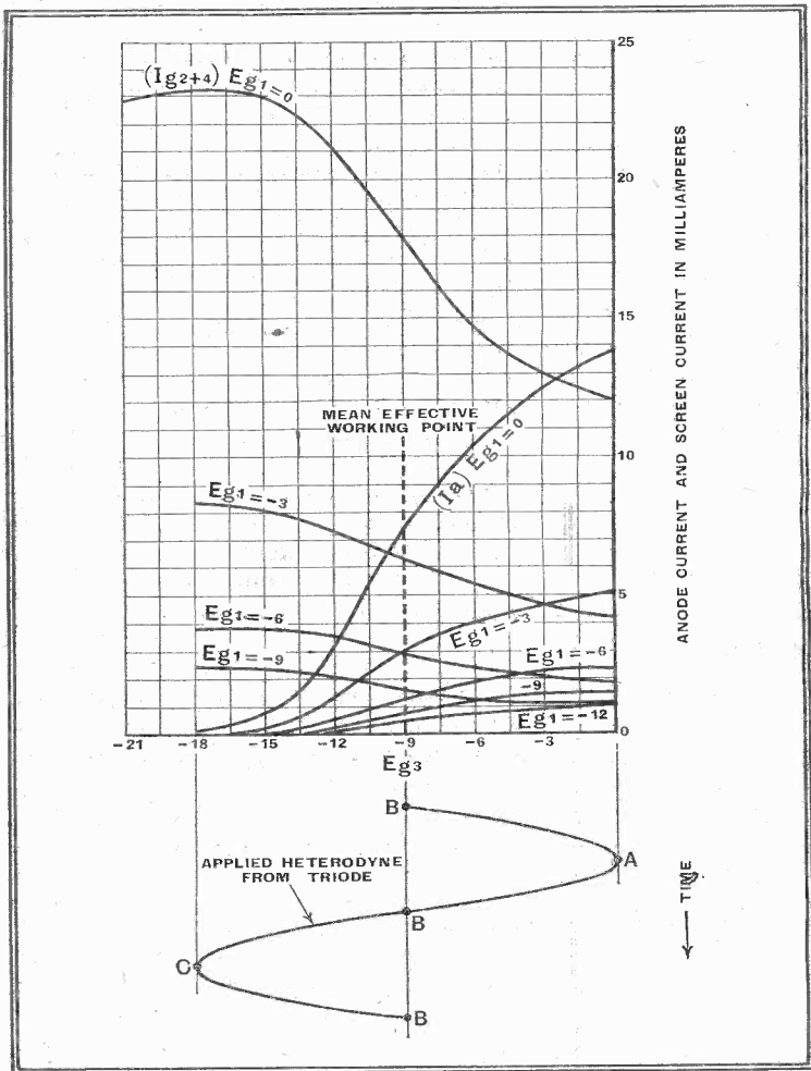
Fig. 2.—Static anode current and accelerator grid current curves of a typical triode-heptode taken as a function of the injector-grid voltage. The bottom half of the figure shows the heterodyne wave in a time-distance sense. The three cardinal points are (A) maximum positive peak; (B) mean effective voltage; and (C) maximum negative peak.
