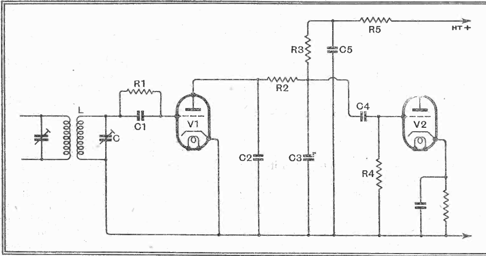
Fig. 2. The grid detector usually takes this form. The valve V1 really functions as a combined diode detector and AF amplifier.
