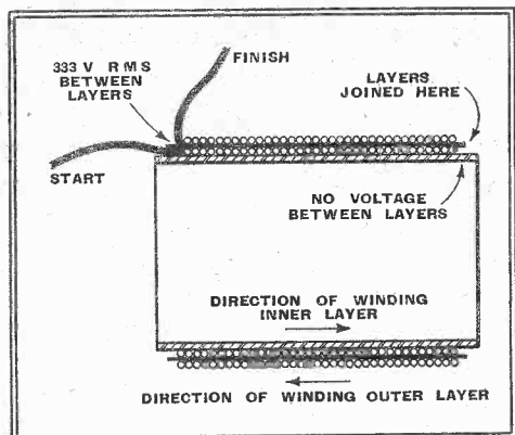
Fig. 1.—The voltage between layers varies from zero at one end to double the voltage per layer at the other end.
