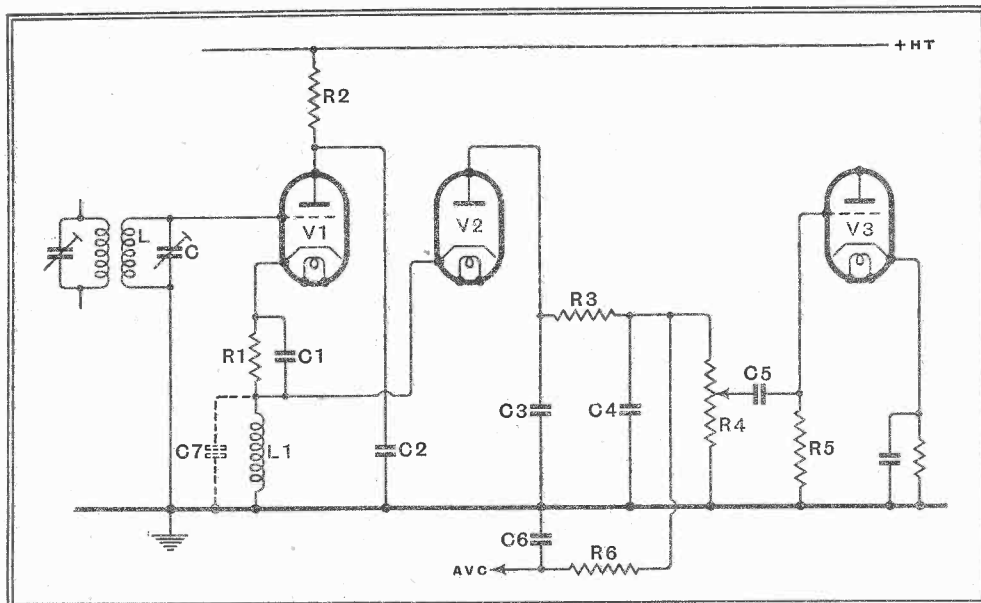
Fig. 5.—This diagram shows the diode detector V2 fed from a cathode-follower V1. By including C7 regeneration can be secured. V3 is an AF stage.
