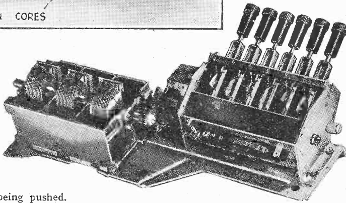
(Above) Iron-cored adjustable inductances for Telefunken push-button superhet.
